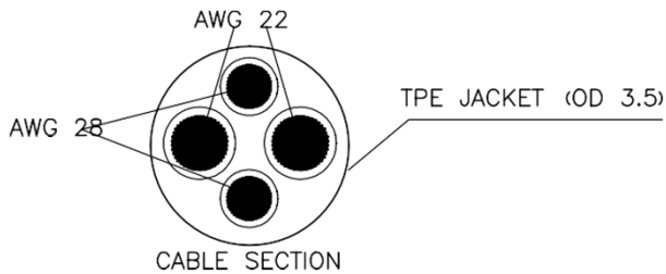
CABLE SECTION
